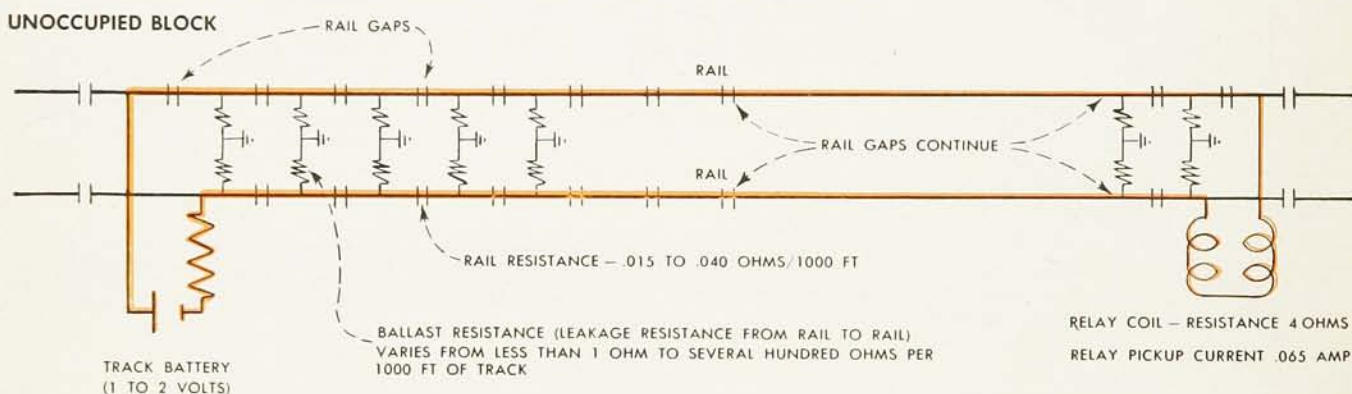
FIG 4 TYPICAL TRACK CIRCUIT CONDITIONS
