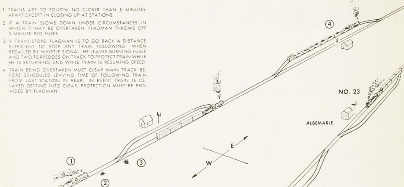
FIG 1 ESSENTIALS OF TIMETABLE AND TRAIN ORDER OPERATION
