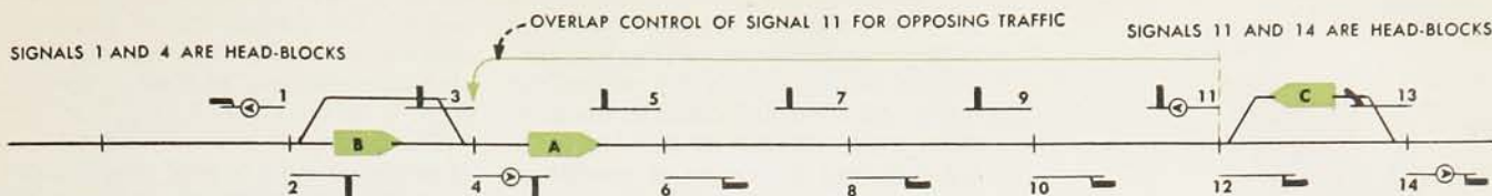
FIG 14 ABSOLUTE PERMISSIVE BLOCK SIGNALING
