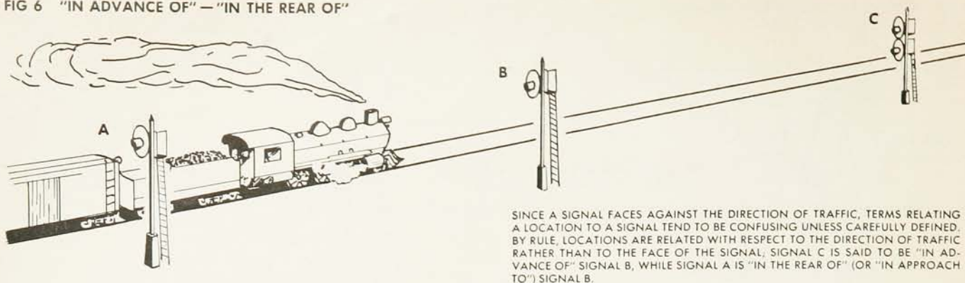
FIG 6 "IN ADVANCE OF" — "IN THE REAR OF"
